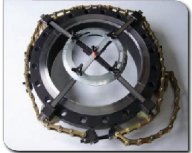
TU 1100 PORTABLE MACHINING UNIT WITH FC 1150 KIT
